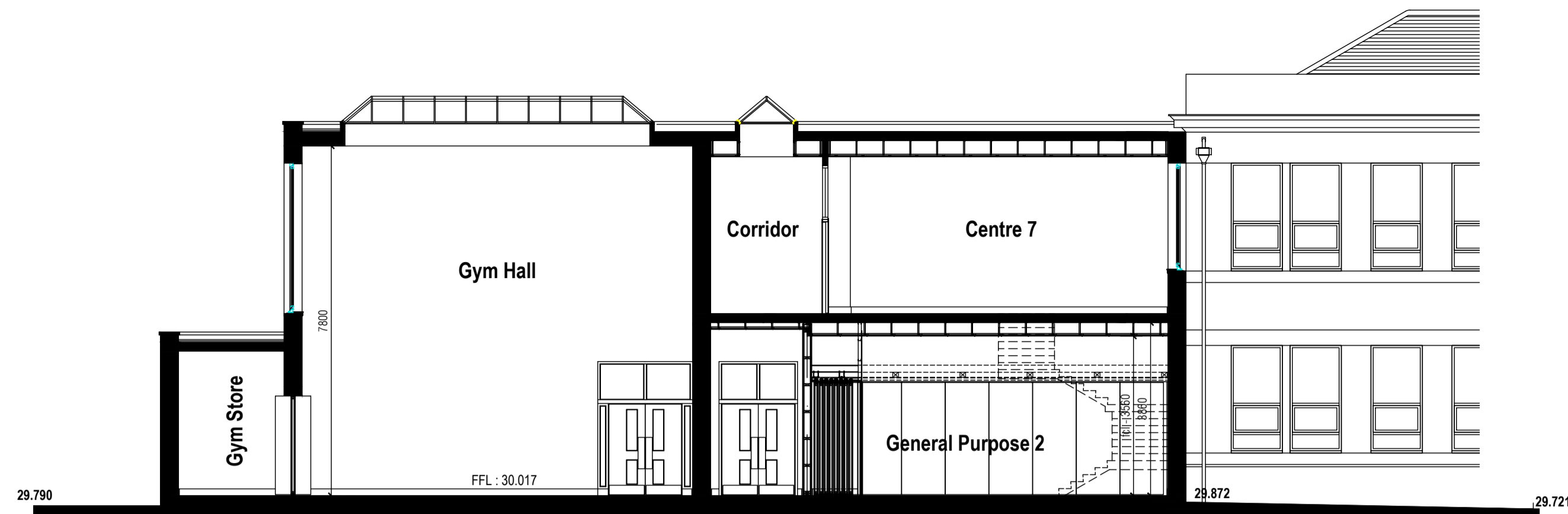
CROSS - SECTION D - D
