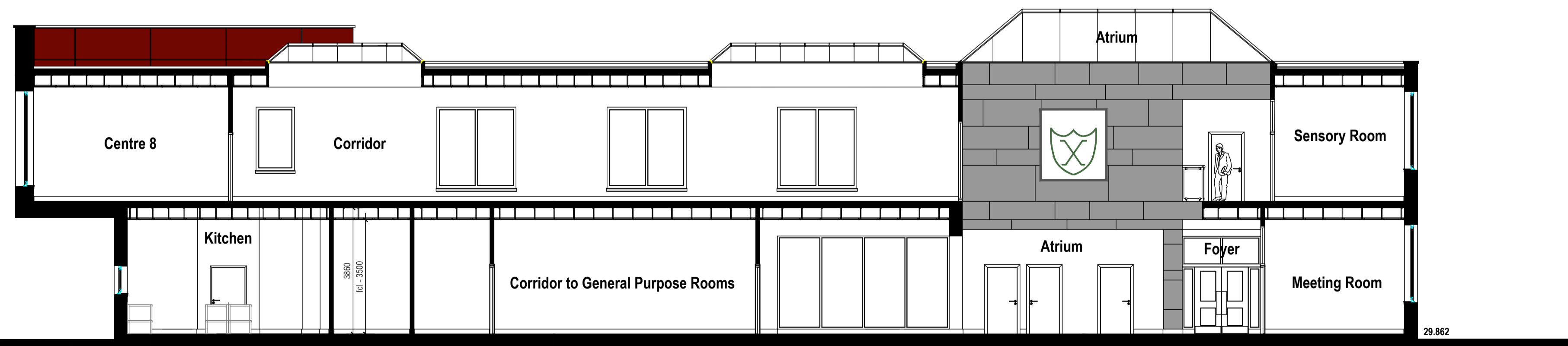
CROSS - SECTION F - F
